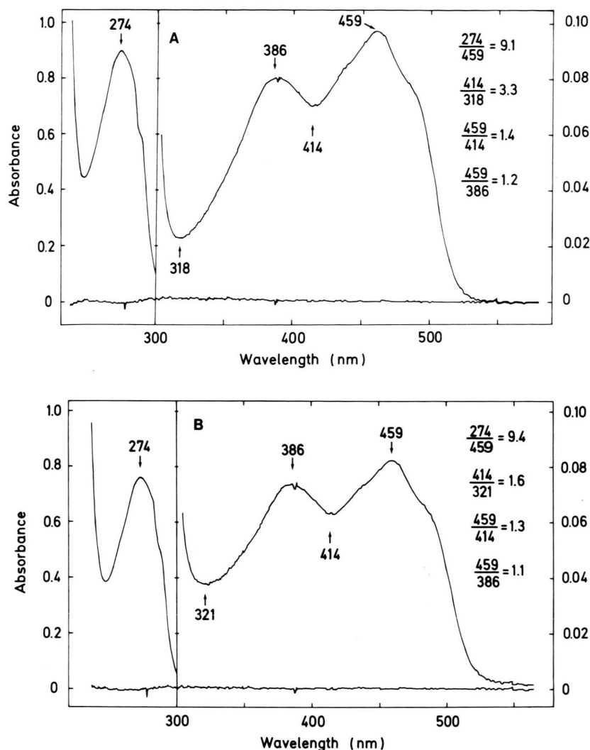
Fig. 3 A, B. Absorption spectra of the 38,000 dalton (A) and 80,000 dalton (B) enzyme species recorded after their elution from the Sephadex G-150 column (Spectrophotometer, Varian Super-Scan 3; protein dissolved in elution buffer as in Fig. 1 A, which also served as reference).
